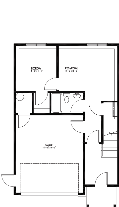
LOWER FLOOR= 595 SQ.FT. GARAGE = 350 SQ.FT.
