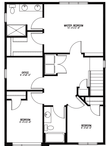
UPPER FLOOR = 968 SQ.FT.
